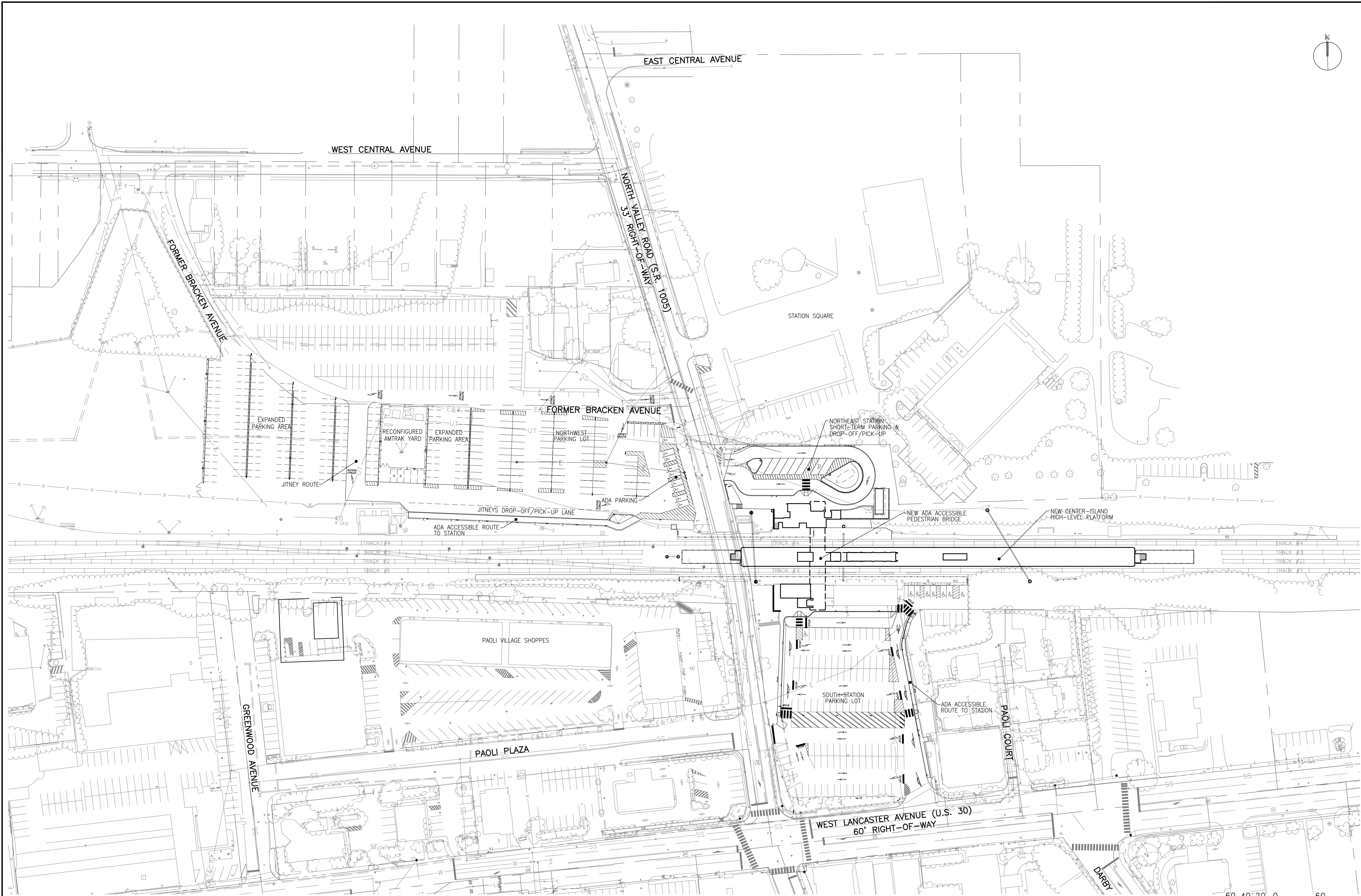
1 OVERALL SITE PLAN SCALE: 1"=60'
